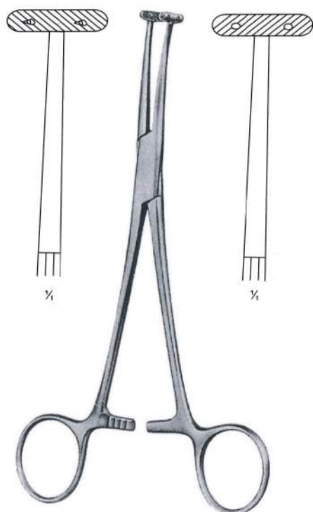
Willet-Martel Haemostatic Forceps MB6 - 264 19.0 cm , 7 1/2"
